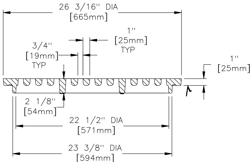
GRATE SECTION
