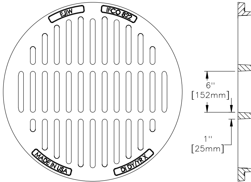
GRATE SECTION
