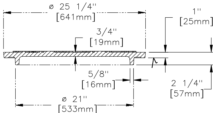
SECTION VIEW
